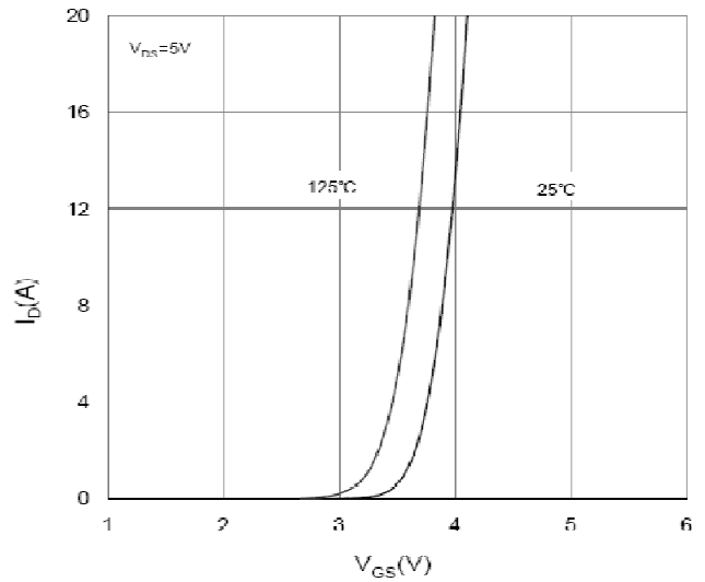
Transfer Characteristic
