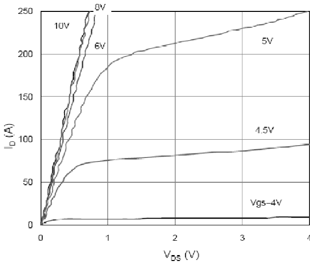
Output Characteristic
